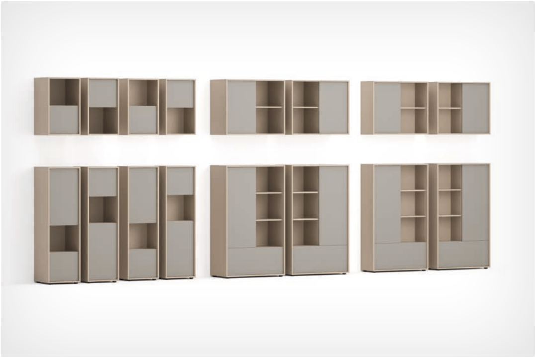
Dimensioni Echo pensile / Echo wall-fixed dimensions: L. / W.45-90-120cm H.36,8-73,6-110,4cm P. / D.32,8-45,6cm Dimensioni Echo a terra / Echo floor-standing dimensions: L. / W.45-90cm H.147,2cm P. / D.45,6cm
